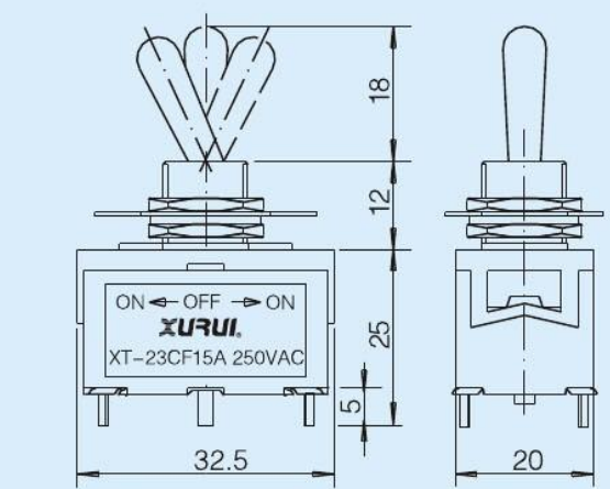
• 双极双向自动复位型 DPDT REINICIO AUTOMATICO (ON)-OFF-(ON) XT-23CF
