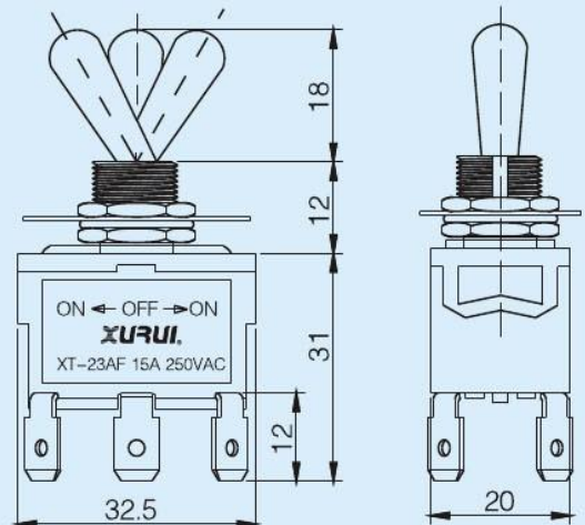
• 双极双向自动复位型 DPDT REINICIO AUTOMATICO (ON)-OFF-(ON) XT-23AF
