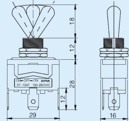
• 单极双向自动复位型 SPDT REINICIO AUTOMATICO (ON)-OFF-(ON) XT-13AF
