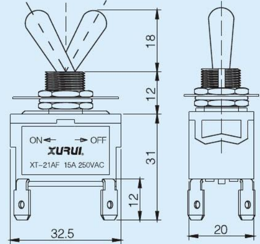
• 双极单向自动复位型 DPST REINICIO AUTOMATICO (ON)-OFF XT-21AF
