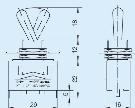
• 单极单向自动复位型 SPST REINICIO AUTOMATICO (ON)-OFF XT-11CF
