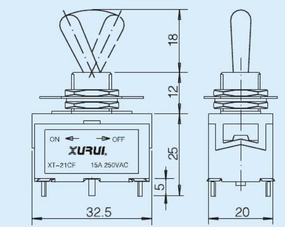
• 双极单向自动复位型 DPST REINICIO AUTOMATICO (ON)-OFF XT-21CF
