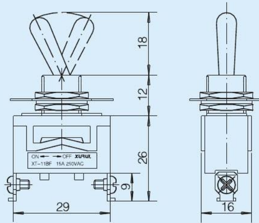
• 单极单向自动复位型 SPST REINICIO AUTOMATICO (ON)-OFF XT-11BF
