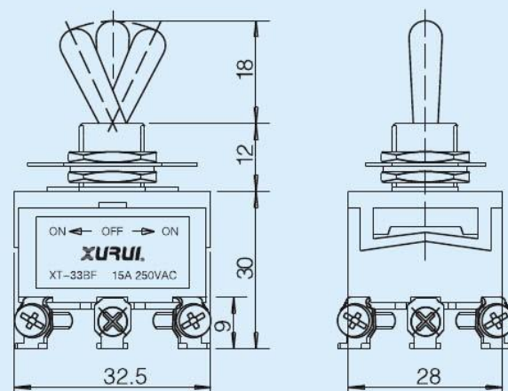
• 三极双向自动复位型 TPDT REINICIO AUTOMATICO (ON)-OFF-(ON) XT-33BF
