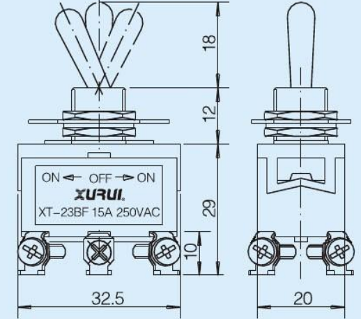
• 双极双向自动复位型 DPDT REINICIO AUTOMATICO (ON)-OFF-(ON) XT-23BF
